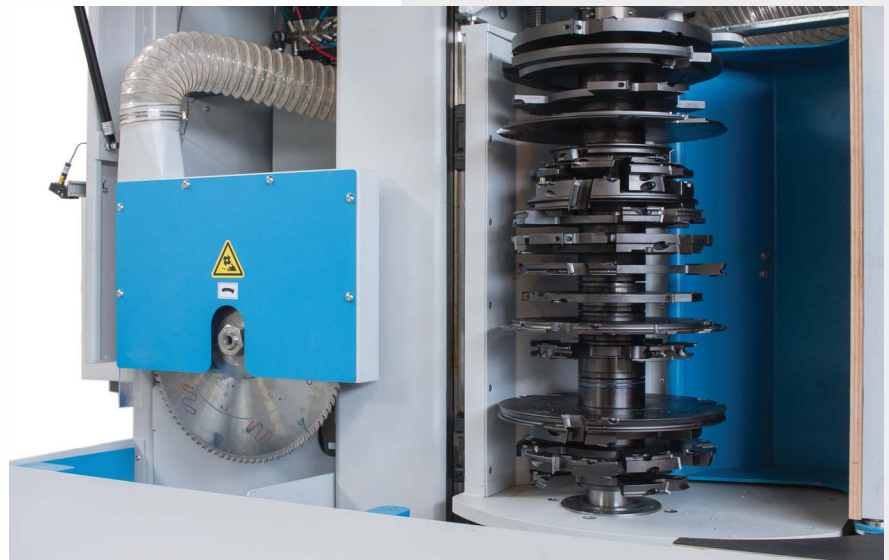
Chip breaking device for tenoning
