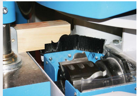
Horizontal milling unit for horns and trenching operations
