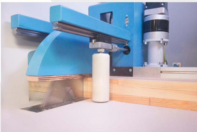
side and top clamp for precise cut
